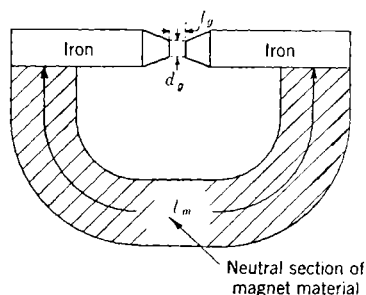
FIG. 13-1.—General type of magnetic circuit.
